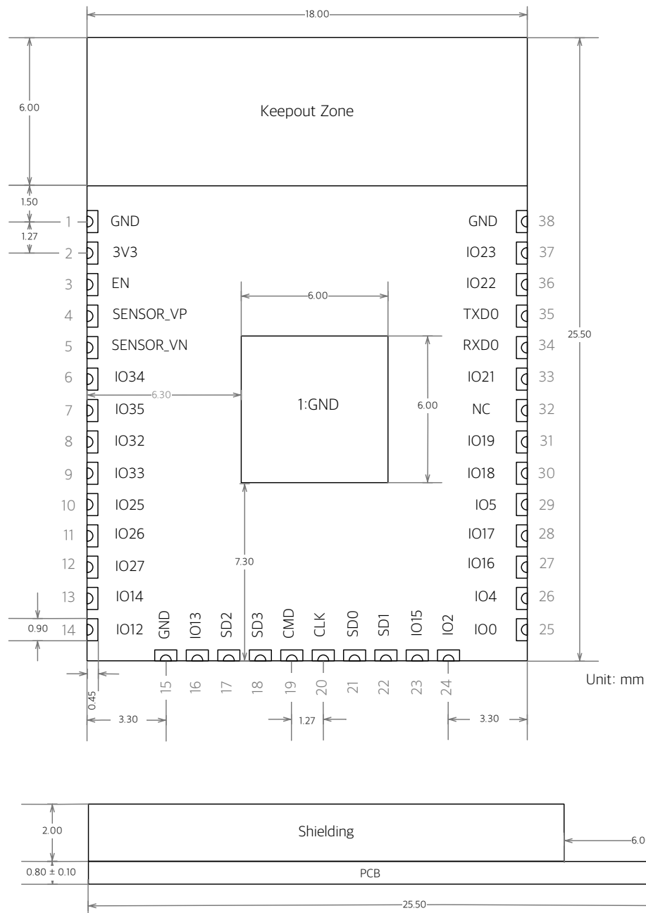
Figure 1: Top and Side View of ESP-WROOM-32
